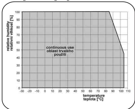
Figure: Working range of Ethernet sensor
