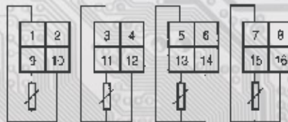
Two-wire connection Ni1000, Pt1000, OV 100, OV 105
